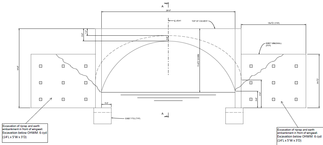
CULVERT ELEVATION VIEW
